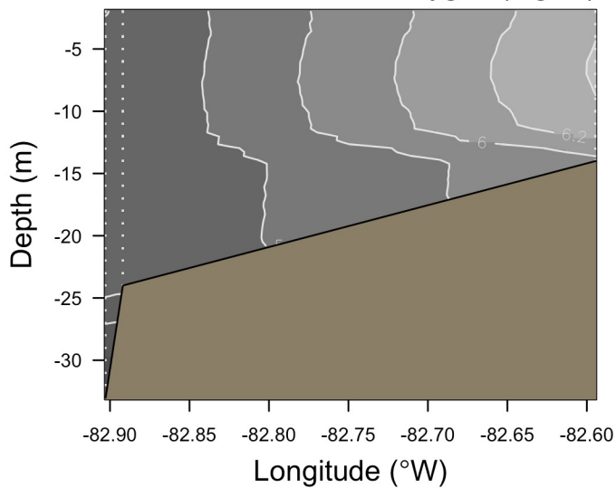
Dissolved Oxygen ( \text{mg l}^{-1} )
