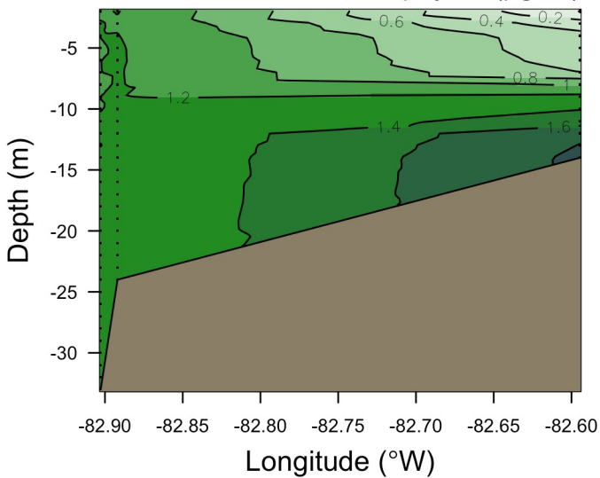
Chlorophyll-a ( \mu\text{g l}^{-1} )
