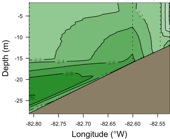
Chlorophyll-a ( \mu\text{g l}^{-1} )
